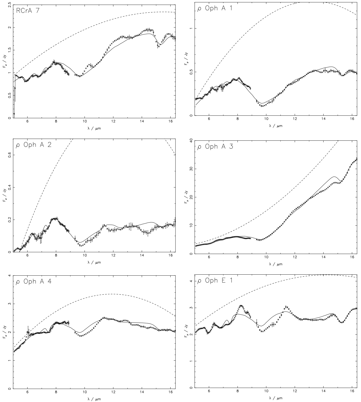
Fig. A.2. Spectra of RCrA 7, \rho Oph A 1-4 and \rho Oph E 1. Note that source \rho Oph A 4 fell on the bad column on the array.
