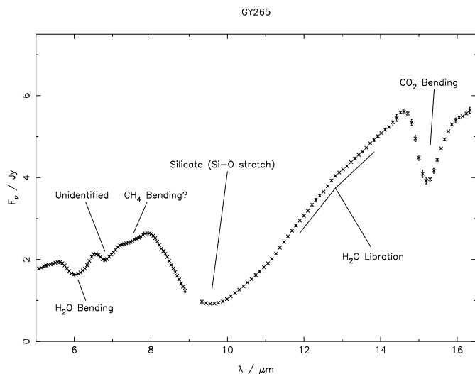
Fig. 1. A typical spectrum, with prominent spectral features annotated.
