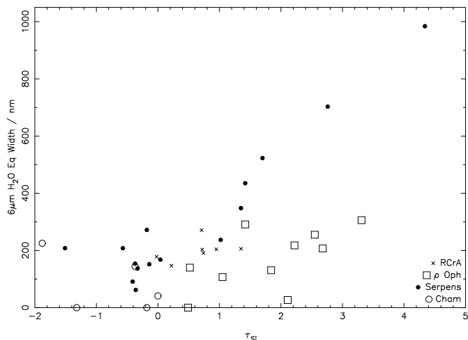
Fig. 8. The strength of the bending mode of water ice plotted against the silicate optical depth. Different regions are distinguished by different symbols, as shown in the legend.
