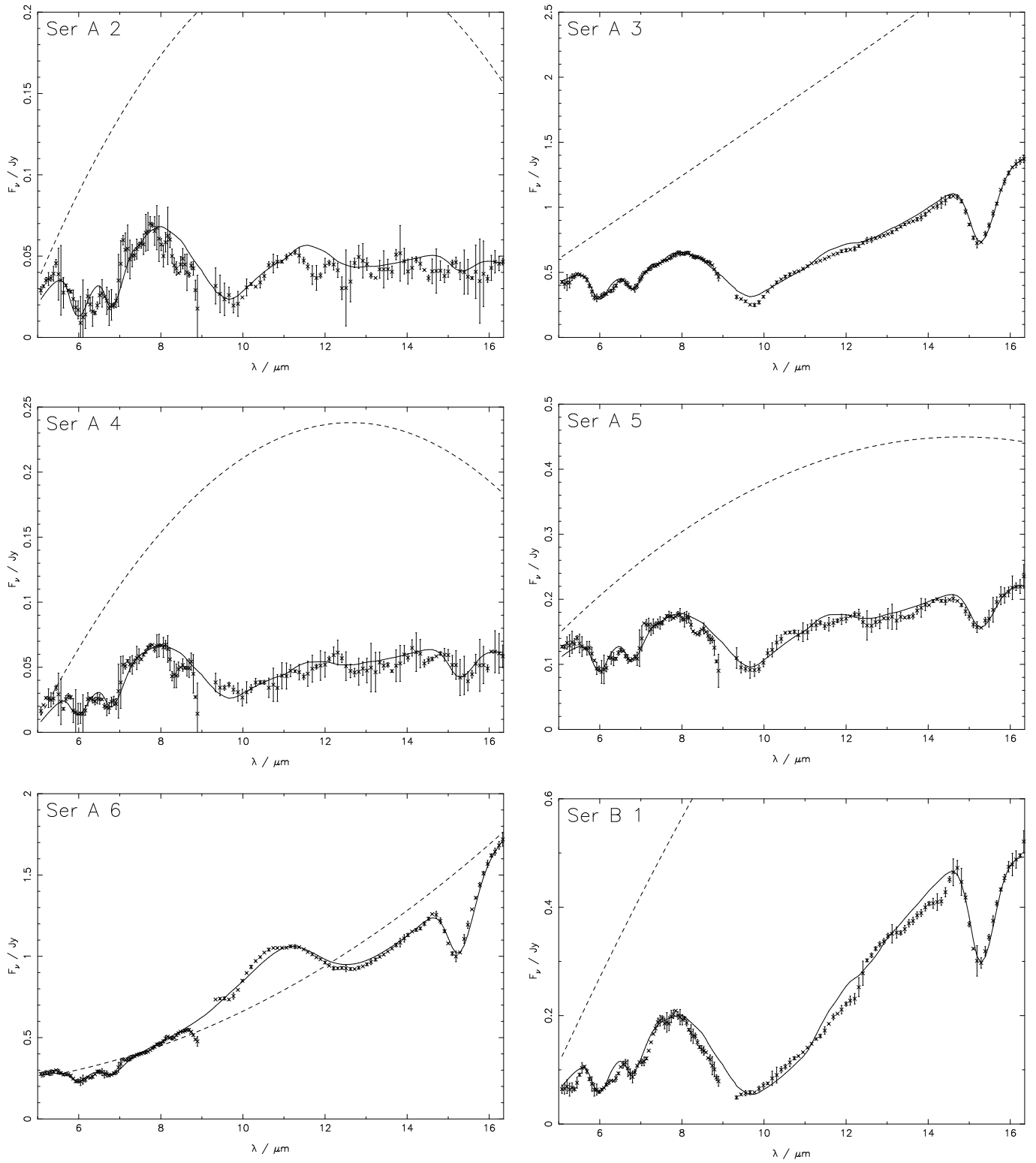
Fig. A.4. Spectra of Ser A 2-6 and Ser B 1. The partial spectrum of Ser A 7 is omitted as a complete spectrum of the same object was found as Ser B 11. Note also that both Ser A 3 and 6 were found to be unresolved doubles.
