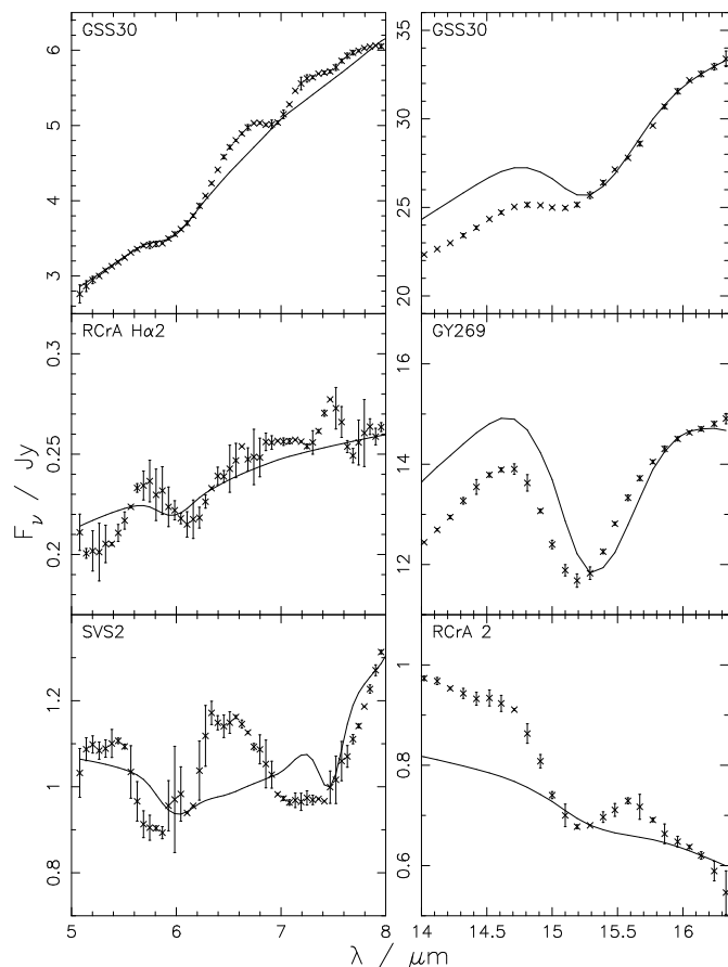
Fig. 3. Examples of poor fits (solid lines) from 5–8 \mu m and around the CO 2 ice feature.
