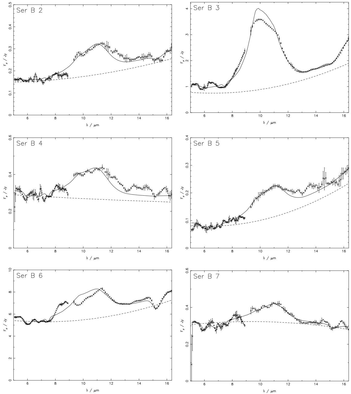
Fig. A.5. Spectra of Ser B 2-7. Note that Ser B 3 and 6 are both unresolved doubles.
