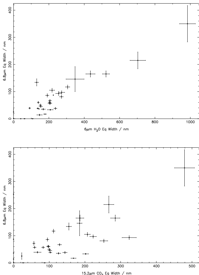
Fig. 5. The strength of the unidentified feature plotted against the bending modes of both water (top) and CO 2 (bottom) ices.
