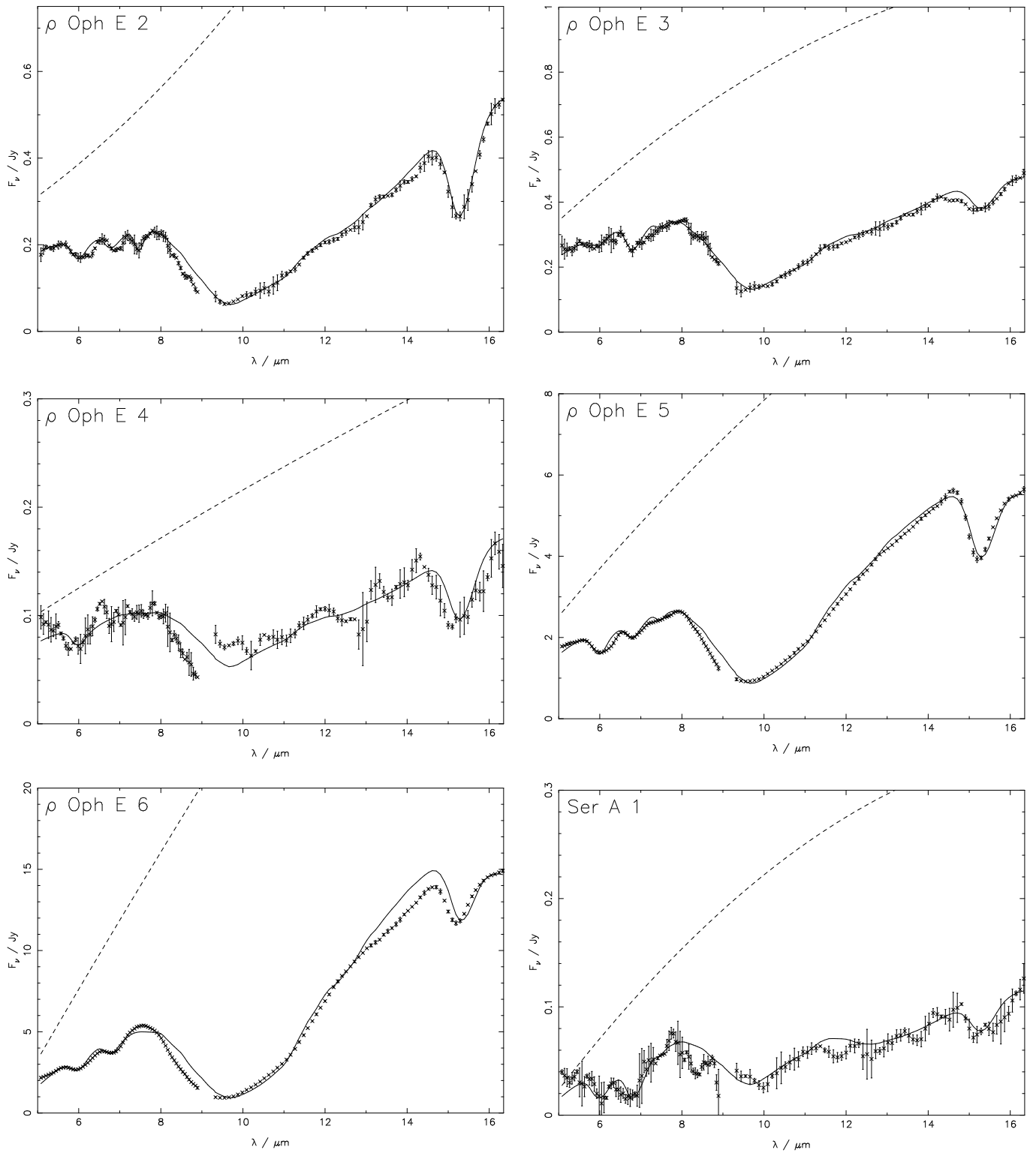
Fig. A.3. Spectra of \rho Oph E 2-6 and Ser A 1.
