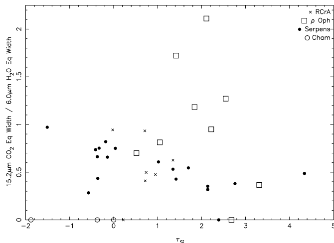
Fig. 9. The ratio of the \text{CO}_2:\text{H}_2\text{O} ice equivalent widths plotted against silicate optical depth. This ratio is directly proportional to the ratio of ice column densities: adopting the band strengths from Gerakines et al. (1995) results in an equivalent width ratio of 1 corresponding to a column density ratio of \approx 0.17 .
