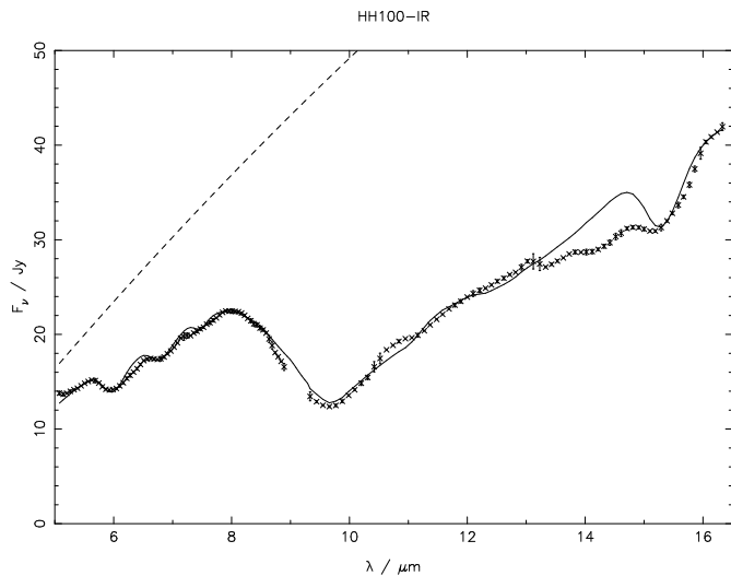
Fig. 4. The spectrum of HH100-IR, with the fitted spectrum (solid line) and continuum (dashed line). Note the poor fit to the CO 2 feature at 15 μm as a further example of why the CO 2 feature was fitted independently.
