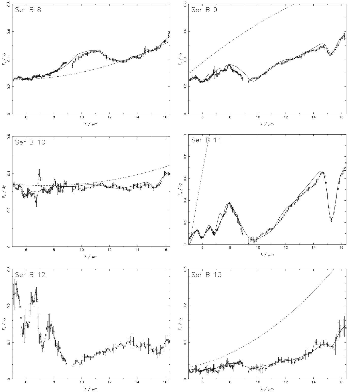
Fig. A.6. Spectra of Ser B 8-13. Source Ser B 8 fell on the bad column of the array, so the data are somewhat dubious. Ser B 12 peaked on the bad column and the resulting spectrum is very poor, so no fit was possible.
