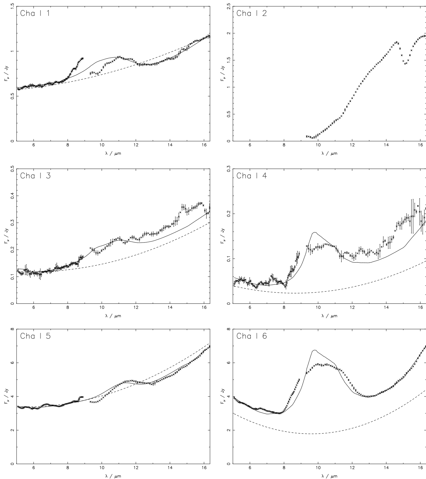
Fig. A.7. Spectra of Cha I 1-6. Cha I 1 fell on the bad column in CVF1, resulting in the large discontinuity seen at the join. Due to the rotation of the spacecraft Cha I 2 was only observed in CVF2.
