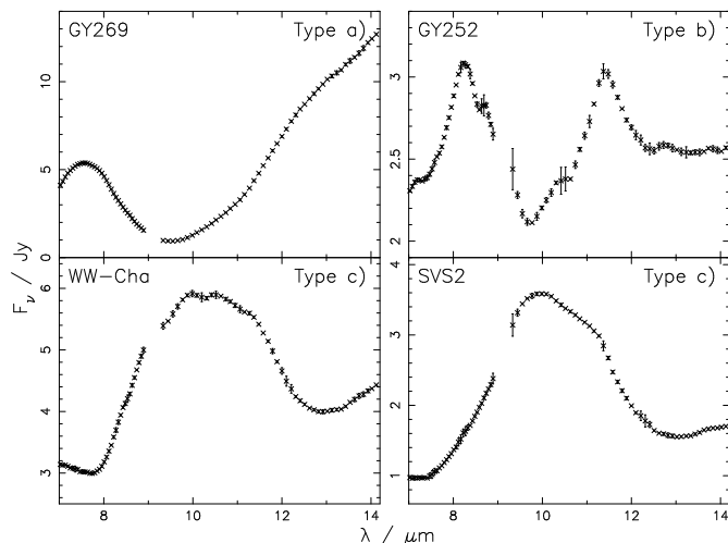
Fig. 6. Examples of observed silicate profiles: emission profiles are generally broader than those seen in absorption and composite emission/absorption profiles are also seen. “Type” refers to the classification scheme described in Sect. 3.2.5.
