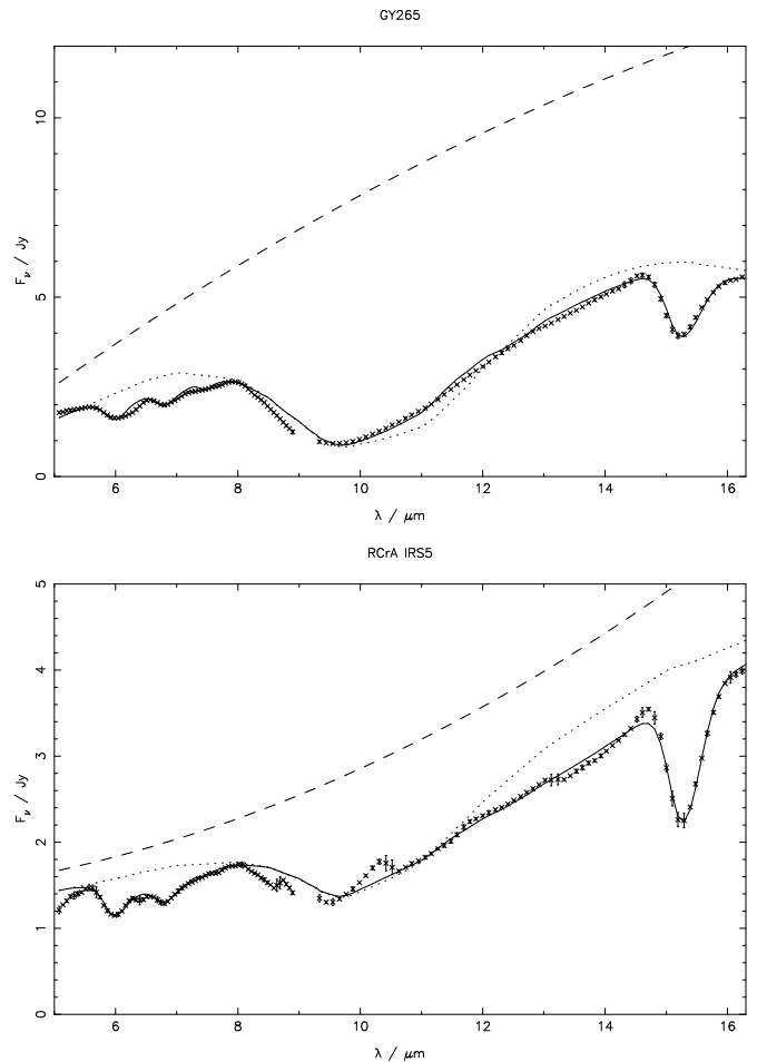
Fig. 2. Examples of successful fits to GY265 in \rho Oph (upper) and RCrA IRS5 (lower): fitted spectra are shown as solid lines and continua as dashed lines. The dotted lines are the “continuum plus silicate” fits given by C(\lambda) \times \exp(-s_{\text{Si}}\alpha_{\text{Si}}(\lambda)) .
