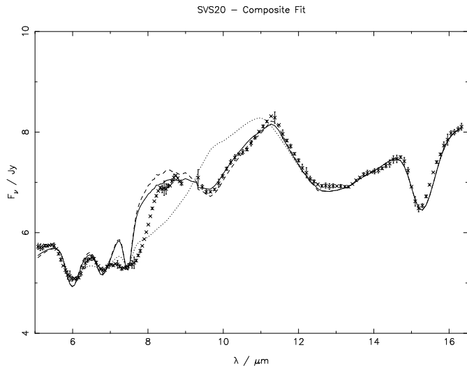
Fig. 7. Composite silicate profiles fitted to the spectrum of SVS20. The solid line shows a composite fit with \tau_{\text{abs}}=0.59 and \tau_{\text{em}}=-0.33 , the dashed line a composite fit with \tau_{\text{abs}}=0.88 and \tau_{\text{em}}=-0.48 (and a different continuum). The single profile fit reported in the results table, with \tau_{\text{Si}}=-0.33 , is shown as the dotted line.
